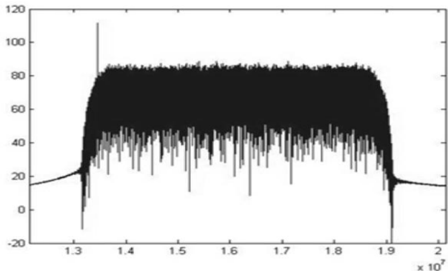
<Drawing 7. outline of the digital TV broadcasting signals >
