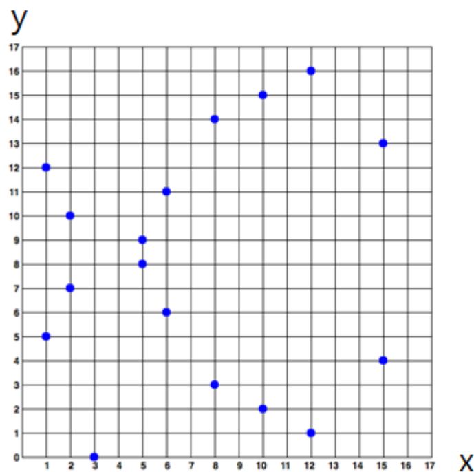
<Drawing 5. A graph that shows x and y coordinates on the elliptic-curve function graph according to the mod p value>
