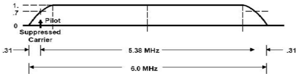
<Drawing 11. the location map of the Pilot signals on the ATSC standards of the digital TV broadcast signals>
