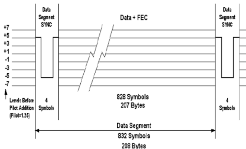
<Drawing 8. the frame structure map of the digital TV broadcast signals >
